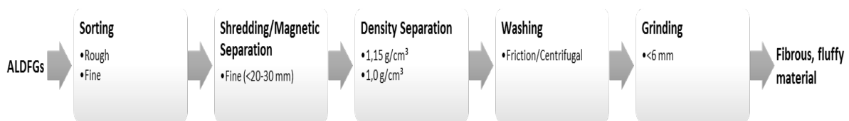
Figure 2: Preparation process for ALDFG tested in MARELITT Baltic with a view to material recycling
