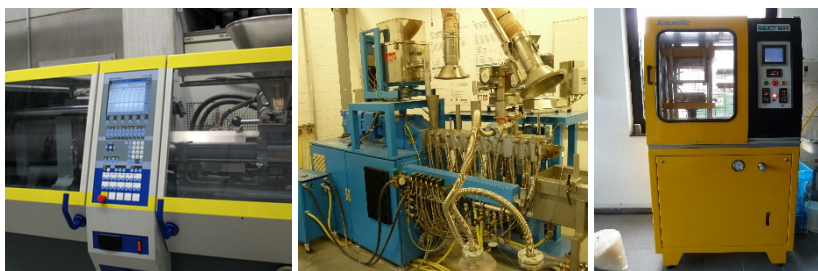
Figure 11: Machines for plastics recycling and downcycling; injection moulding machine (l.), laborextruder (m.), sheet press (r.) (© R. Kopitzky/Fraunhofer UMSICHT)
